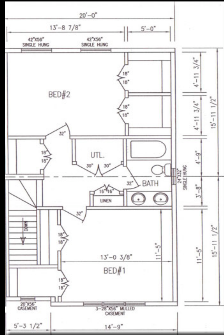
Second Floor
