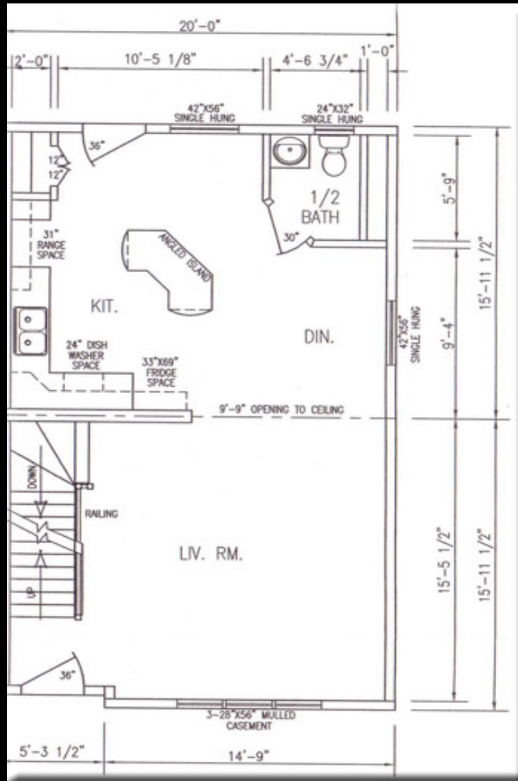
First Floor
